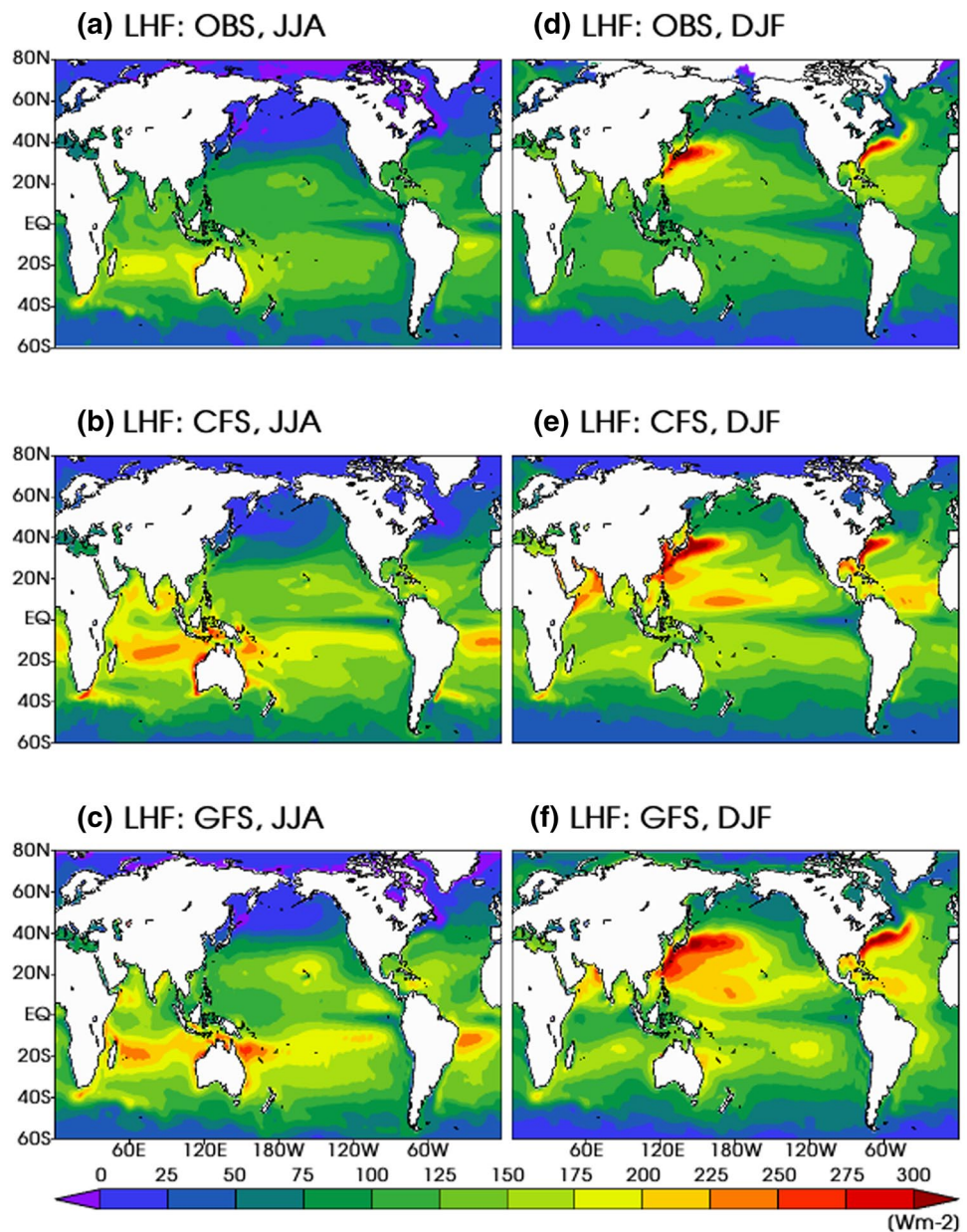
Fig. 6 Seasonal climatology (June–July–August; JJA) of Latent heat flux (LHF) (units: \text{W}/\text{m}^2 ) obtained from a OAFflux, b CFS, and c GFS run for the period 1979–2007. d–f Same as a–c but for DJF season
