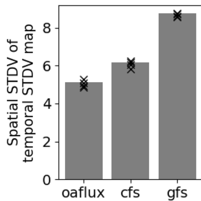
Fig. 11 Spatial standard deviation of the temporal standard deviation map for OAFflux, CFS, and GFS given as Fig. 12a, b, d, respectively (grey bars). The four “x” markers on each bar indicate spatial standard deviation of the temporal standard deviation map as similar to the grey bars but calculated from non-overlapping 7-year chunks (1979–1985, 1986–1992, 1993–1999, and 2000–2006) individually
