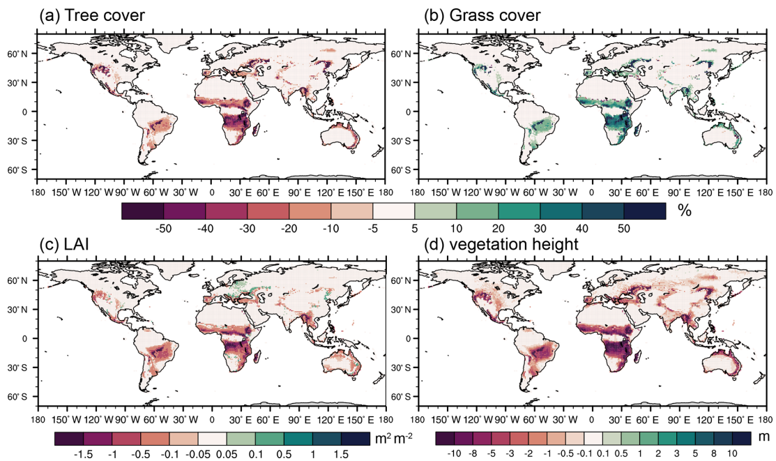
Figure 11. Differences in (a) tree cover (BET, NET, and BDT; %) (b) grass cover (C 3 and C 4 ; %), (c) LAI (m 2 m -2 ), and (d) vegetation height (m) in SSiB4/TRIFFID-Fire averaged over 2000–2014 between FIRE-ON and FIRE-OFF.
